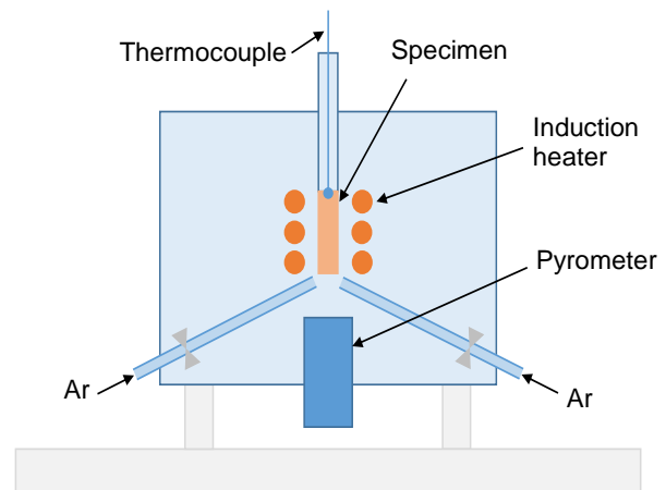
Figure 1: Sketch of the test rig for laboratory scale heat treatment
